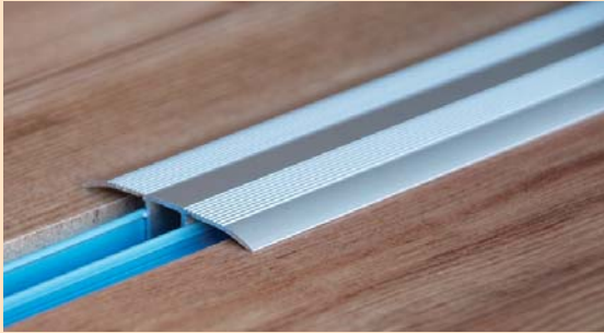
Ktex Motion Profile – Aluminium 7–13mm, Length: 2700mm / 900 mm
